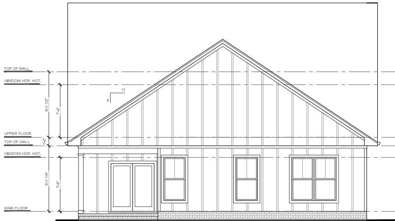
REAR ELEVATION
