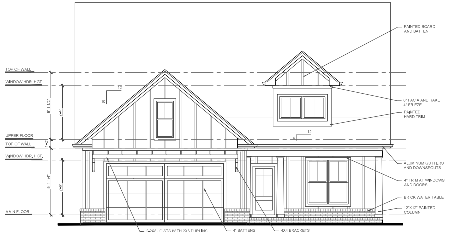
STREET ELEVATION C
