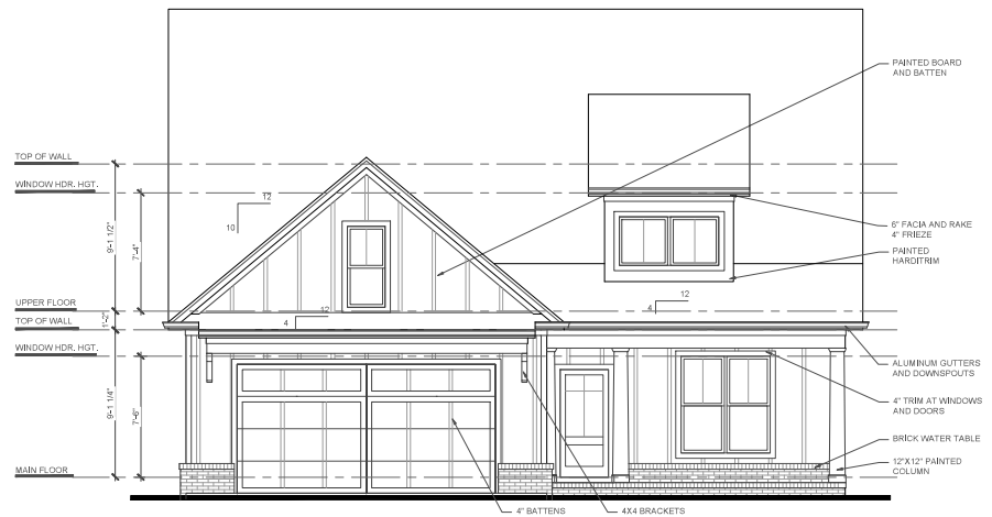
STREET ELEVATION B
