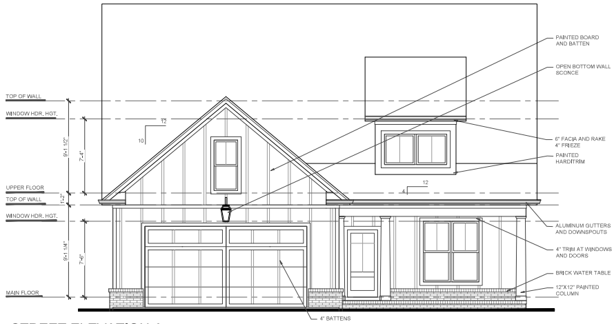
STREET ELEVATION A
